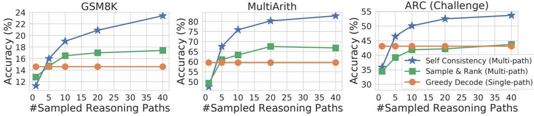
Figure 3: Self-consistency significantly outperforms sample-and-rank with the same # of samples.
